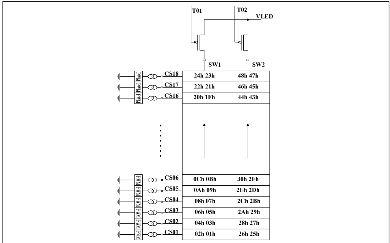
Figure 20 PWM Register
