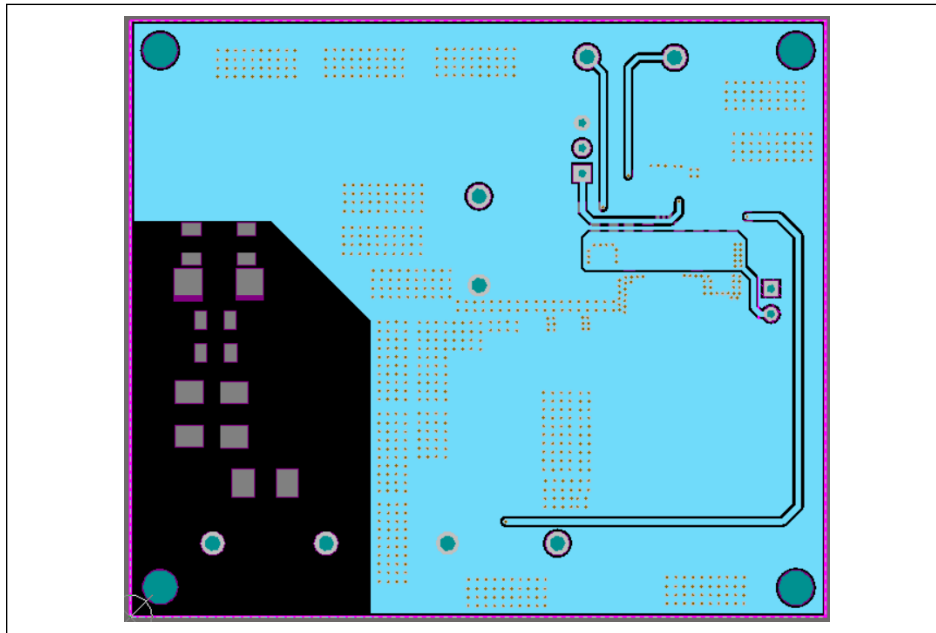
Figure 6 Board PCB Layout - Mid-Layer 2
