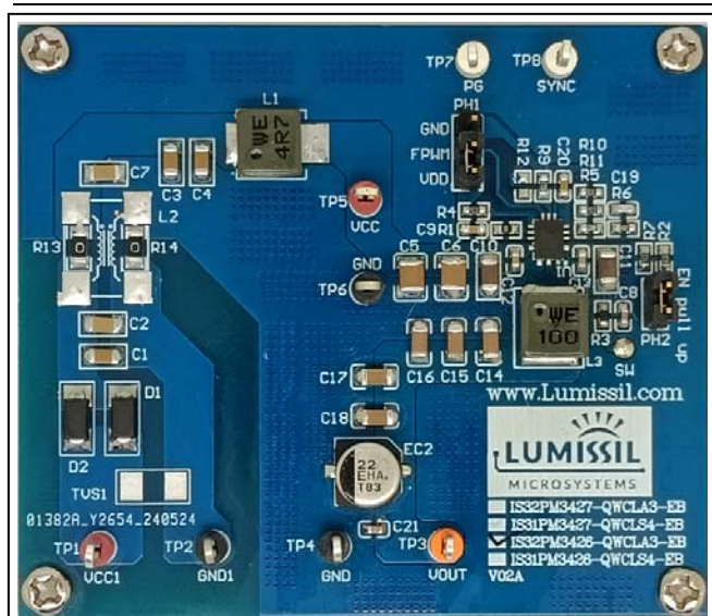
Figure 1 Photo of IS32PM3426 Evaluation Board
