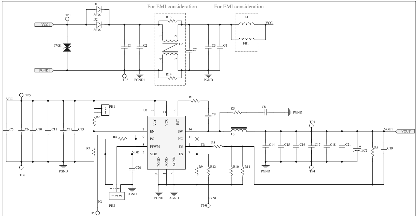
Figure 3 IS32PM3426 Demo Board Schematic
