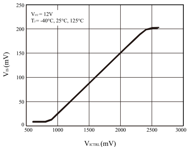
Figure 22 V_{IS} vs. V_{CTRL}
