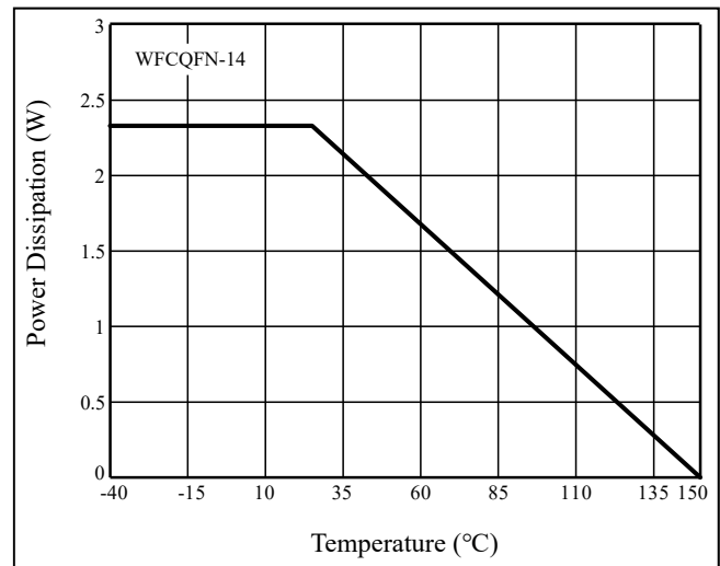
Figure 51 Dissipation Curve
