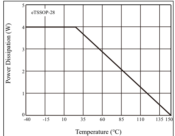
Figure 61 Dissipation Curve
