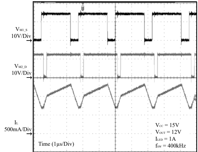
Figure 29 Switching Waveforms (Buck-Boost Region)
