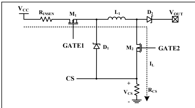
Figure 50 Boost Peak Current Detection in M_2 On Phase
