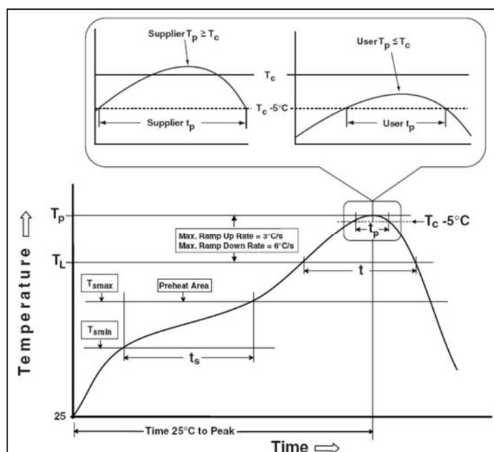
Figure 62 Classification Profile
