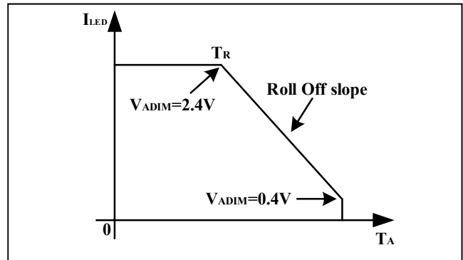
Figure 47 Thermal Roll Off Protection
