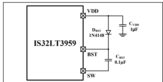
Figure 38 External BST Diode
