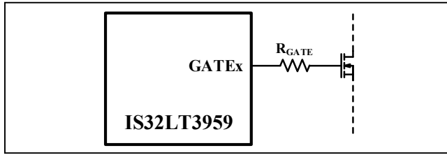
Figure 54 GATE Buffer Resistor
