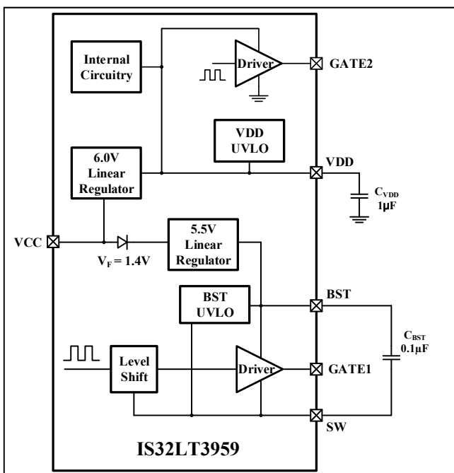
Figure 37 Linear Regulator
