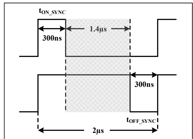
Figure 40 SYNC Pulse On And Off Time Requirements
