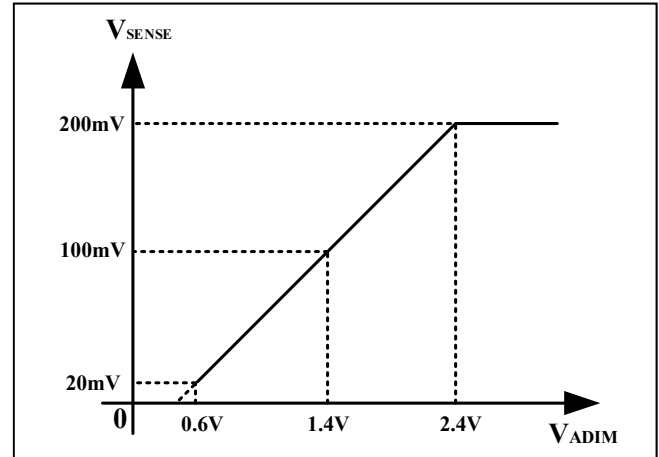
Figure 43 Analog Dimming
