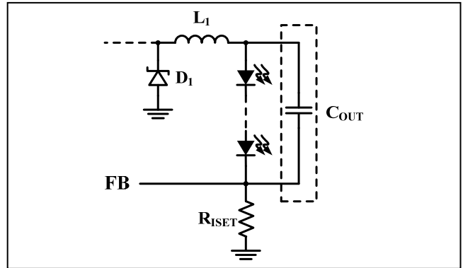
Figure 28 Adding Output Capacitor
