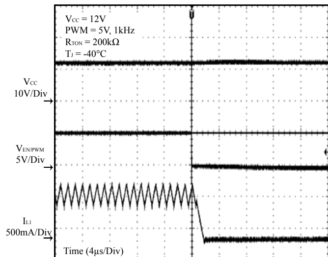
Figure 20 PWM Off
