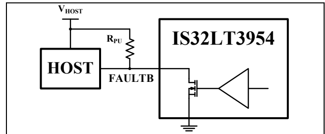
Figure 34 Host Monitors The Fault Reporting
