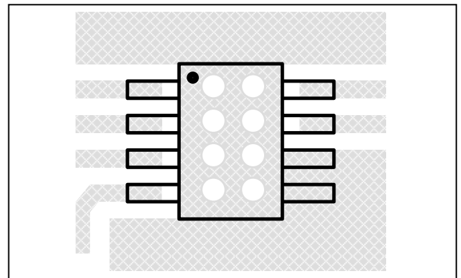
Figure 36 Board Via Layout For Thermal Dissipation
