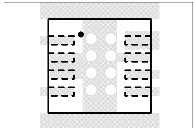
Figure 33 Board Via Layout for Thermal Dissipation (WFDFN package)
