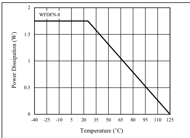
Figure 31 Dissipation Curve
