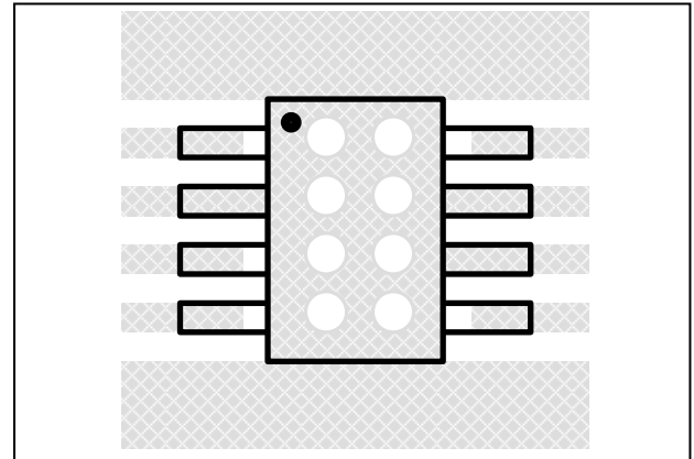
Figure 32 Board Via Layout For Thermal Dissipation (SOP package)
