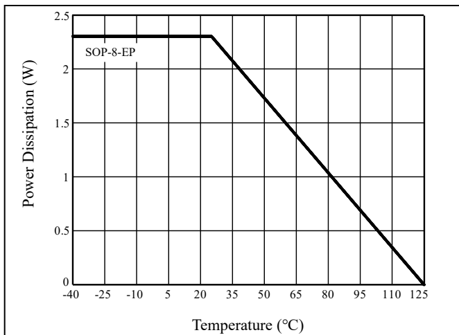
Figure 30 Dissipation Curve
