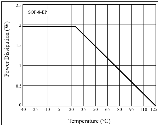
Figure 28 Dissipation Curve
