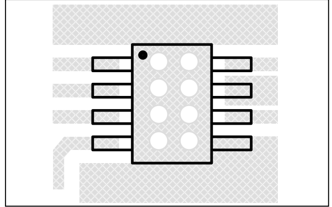
Figure 29 Board Via Layout For Thermal Dissipation
