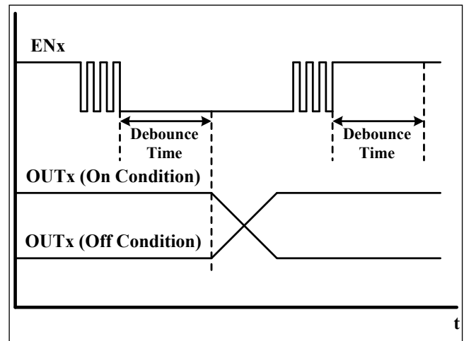
Figure 22 EN Debounced
