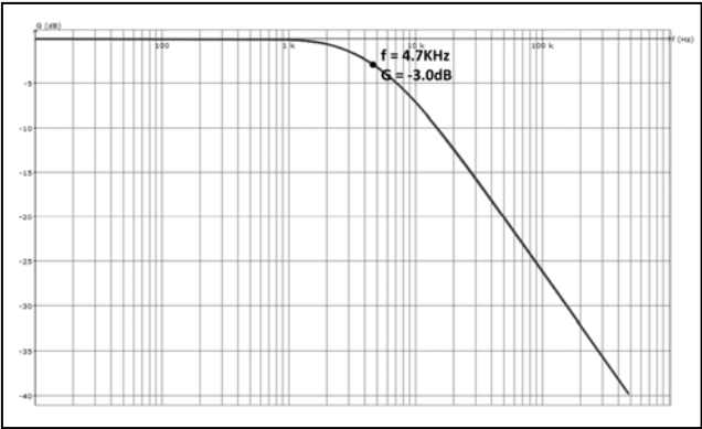
Figure 31 Low-pass filter gain-magnitude frequency response
