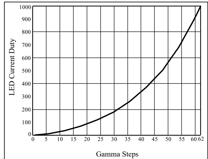
Figure 71 Gamma Correction (63 Steps)
