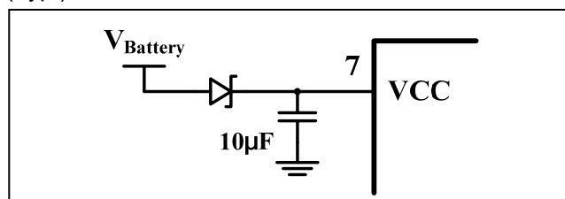
Figure 70 Capacitor For Latch Status
