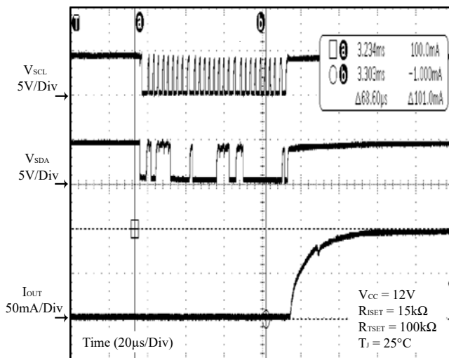
Figure 37 I2C Dimming Rising (T J = 25°C)
