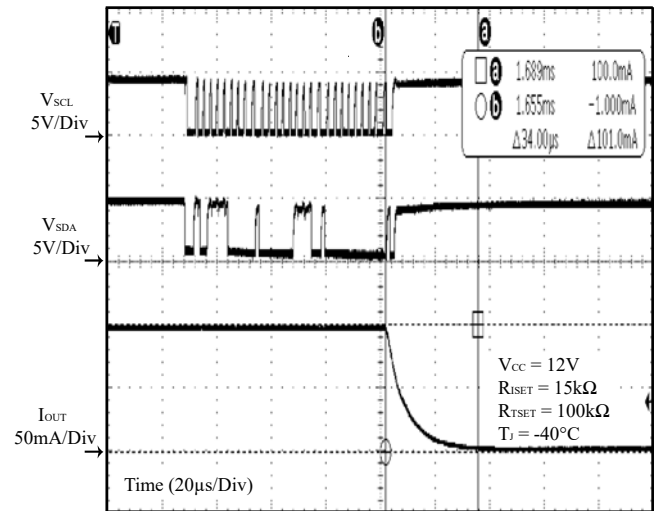
Figure 36 I2C Dimming Falling (T J = -40°C)
