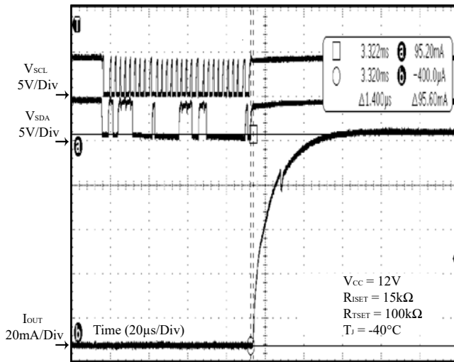
Figure 35 I2C Dimming Rising (T J = -40°C)
