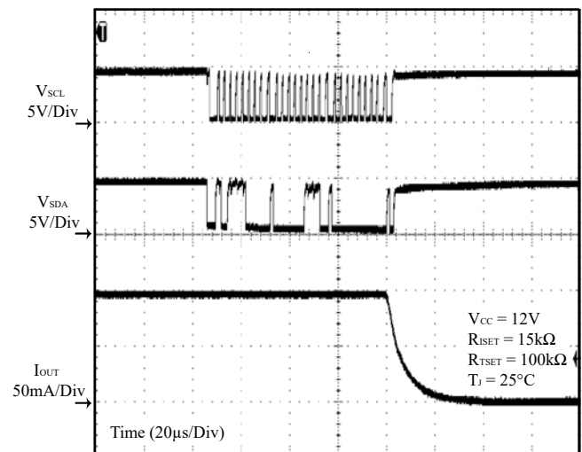
Figure 38 I2C Dimming Falling (T J = 25°C)
