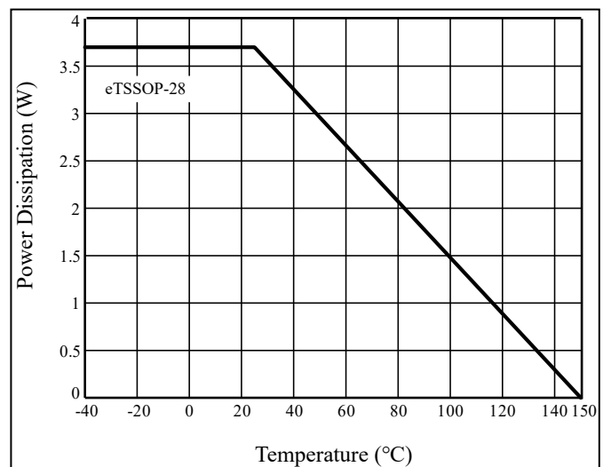
Figure 9 Dissipation Curve
