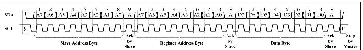
Figure 5 Writing to IS32FL3265A (Typical)
