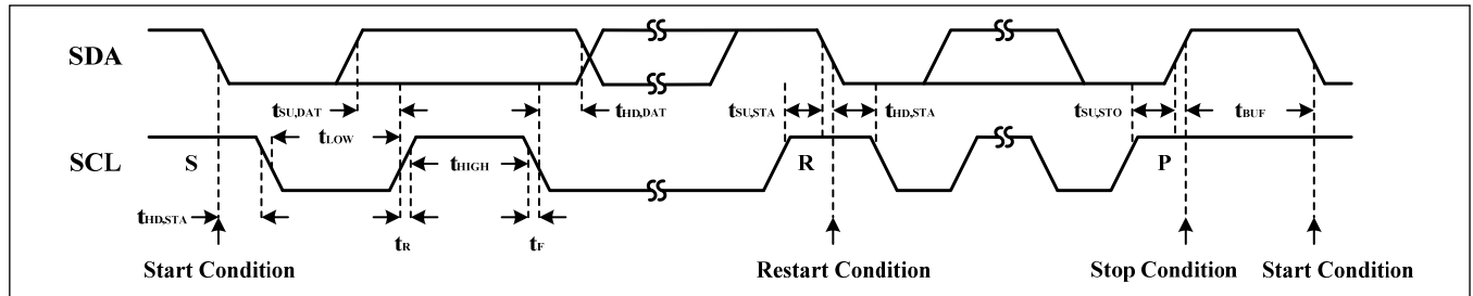
Figure 3 Interface Timing
