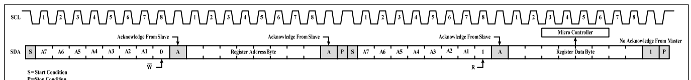
Figure 7 Reading from IS32FL3246A
