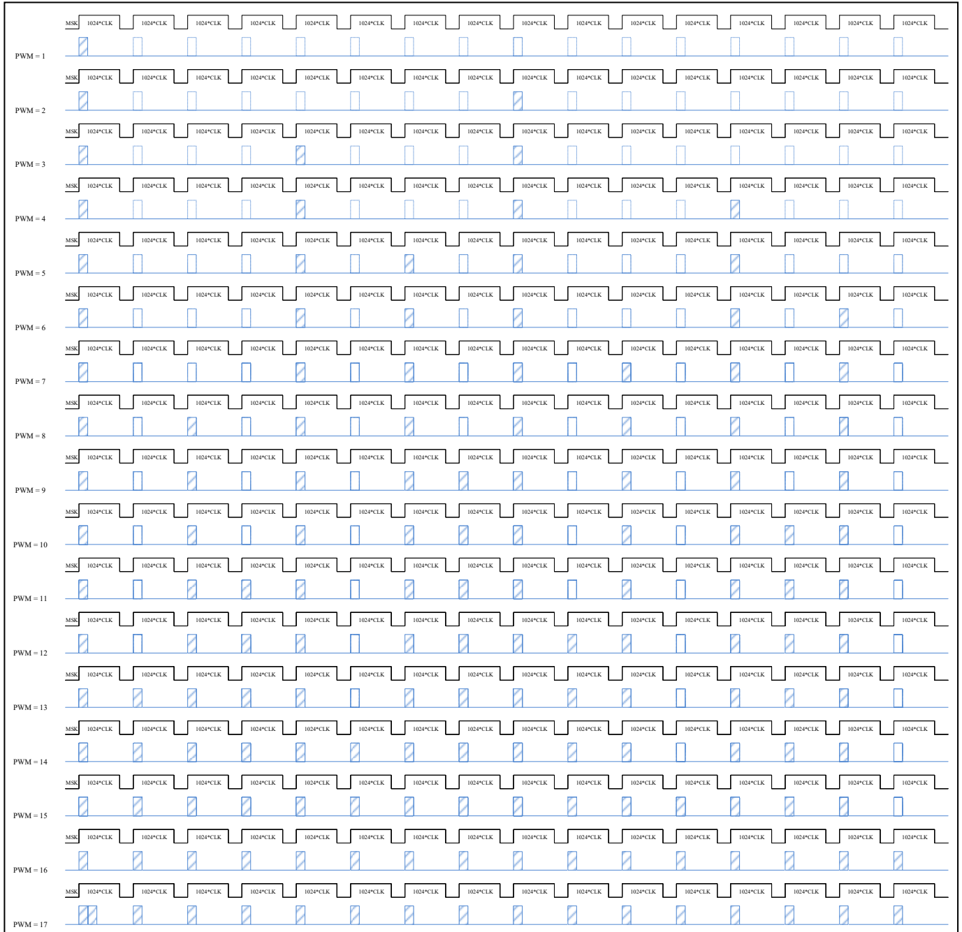
Figure 16 14B_E= "1" 10+4-bit Function Enable
