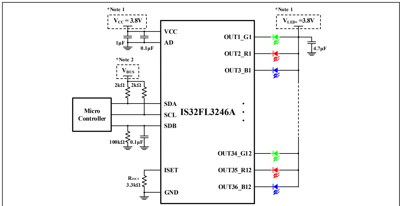
Figure 1 Typical Application Circuit ( V_{CC}=V_{Battery} )
