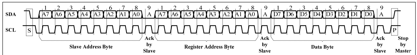
Figure 5 Writing to IS32FL3246A (Typical)
