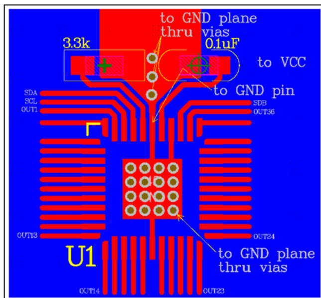
Figure 15 Layout Example
