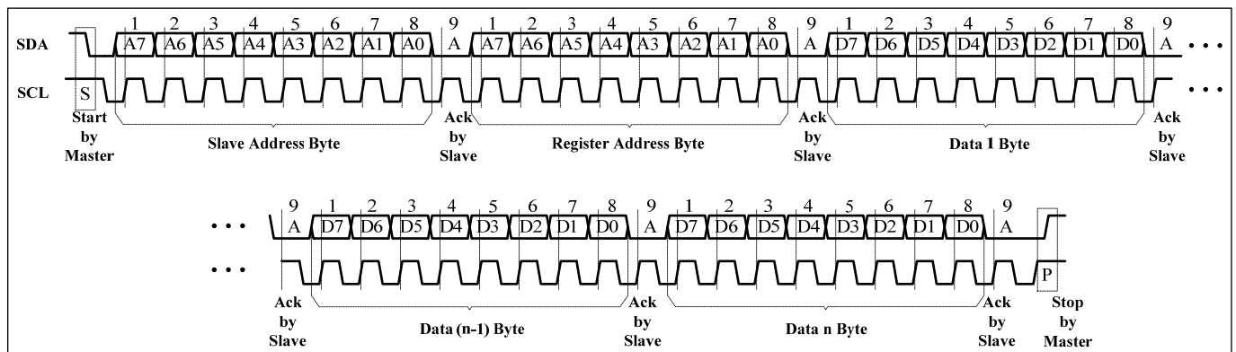
Figure 6 Writing to IS32FL3246A (Automatic Address Increment)
