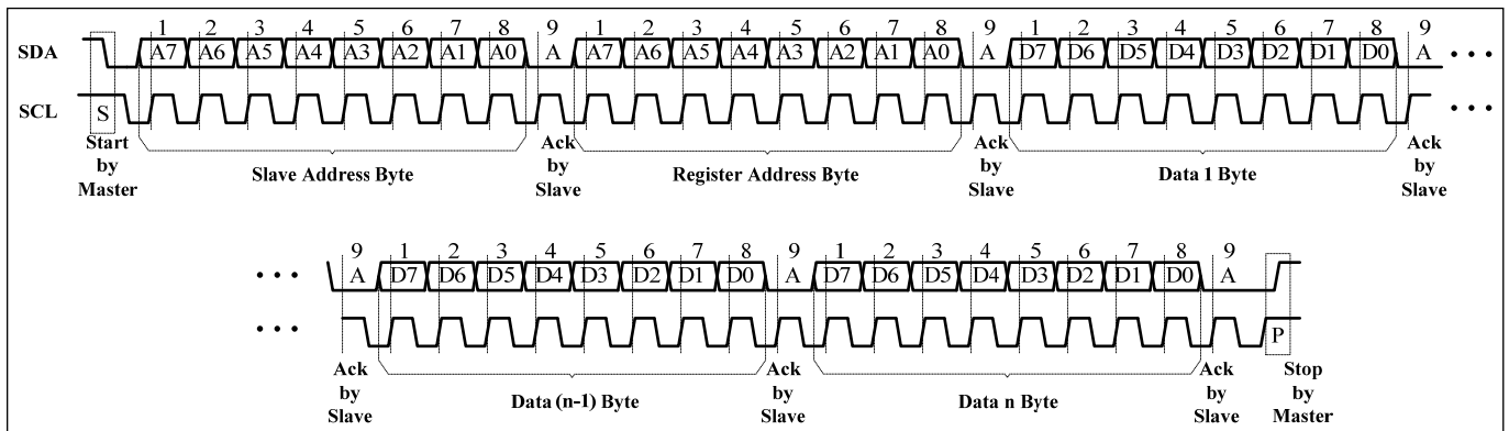
Figure 6 Writing to IS3238 (Automatic Address Increment)
