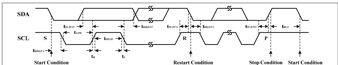
Figure 3 Interface Timing
