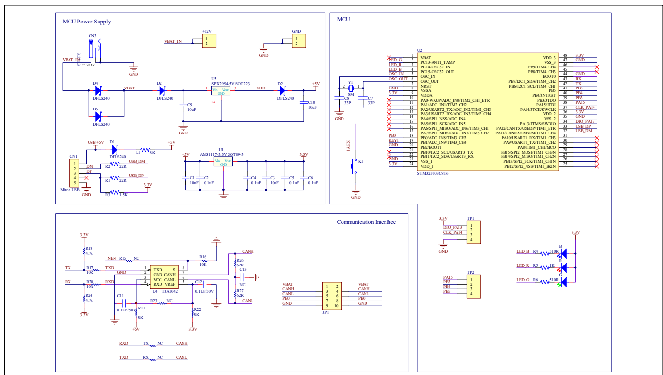
Figure 5 IS32FL3105C MCU EVB Schematic
