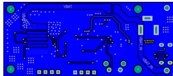
Figure 15 Board PCB Layout - Bottom Layer
