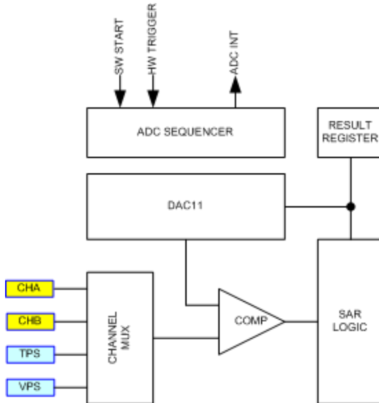
Figure 16-1 11-bit SAR ADC block diagram
