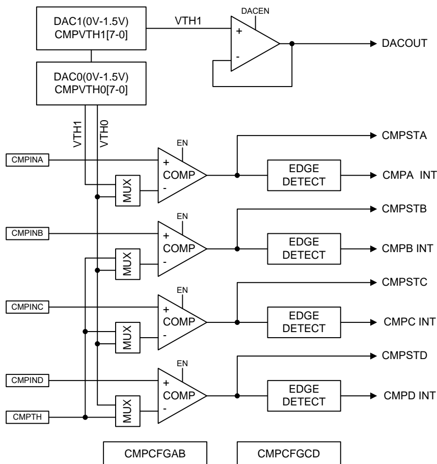
Figure 17-1 ACMP and 8-bit DAC block diagram
