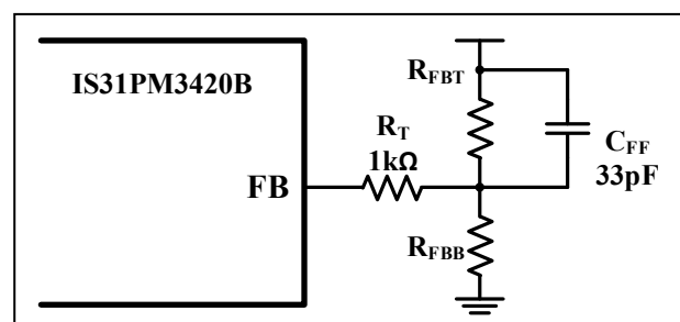
Figure 2 Feedback Network
