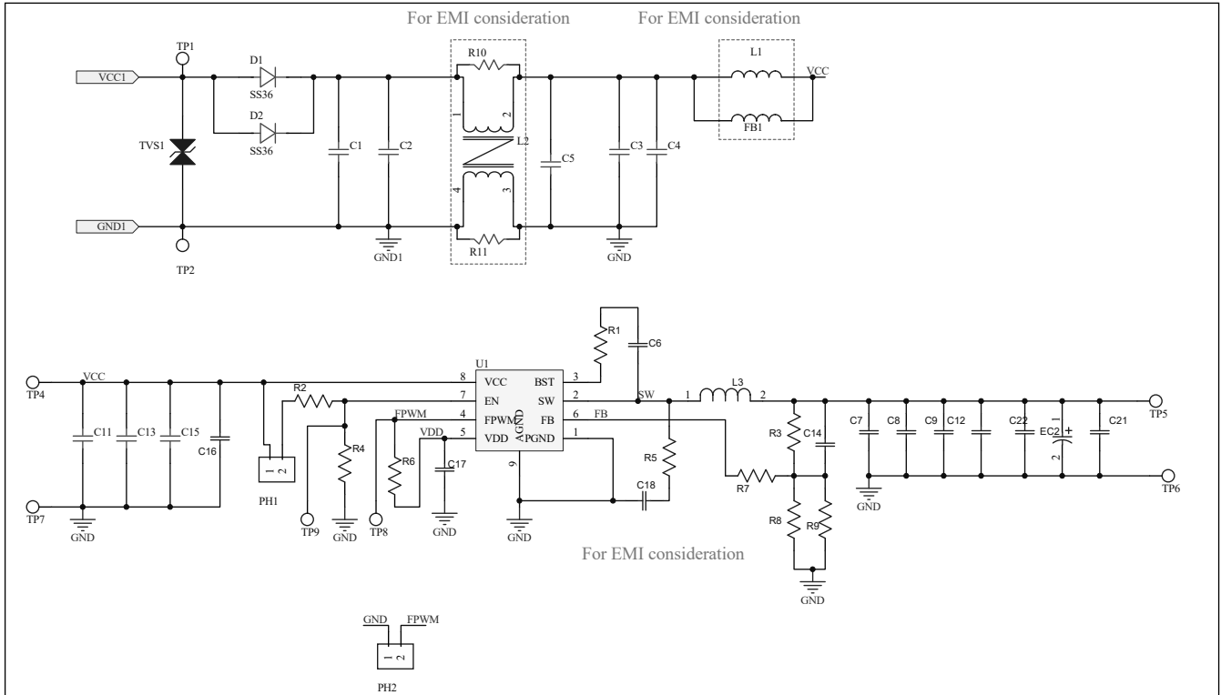
Figure 3 IS31PM3420B Demo Board Schematic
