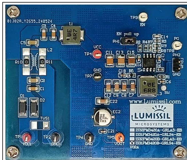
Figure 1 Photo of IS31PM3420B Evaluation Board
