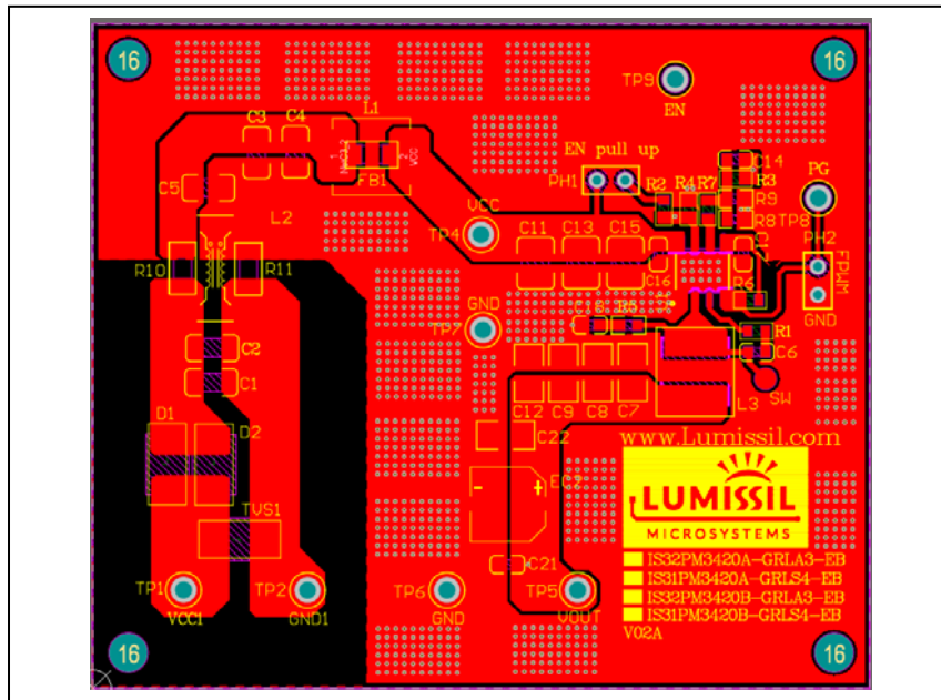
Figure 4 Board PCB Layout - Top Layer
