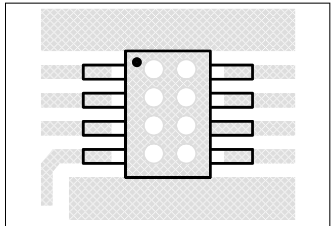
Figure 36 Board Via Layout For Thermal Dissipation
