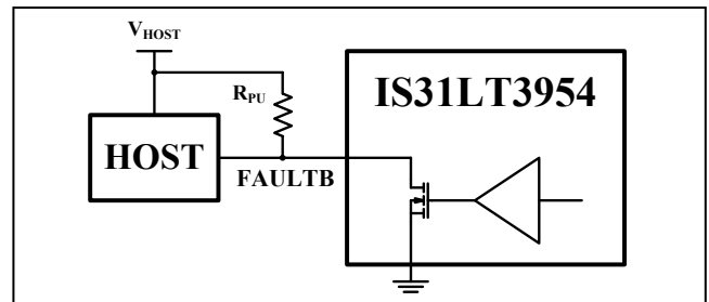
Figure 34 Host Monitors The Fault Reporting
