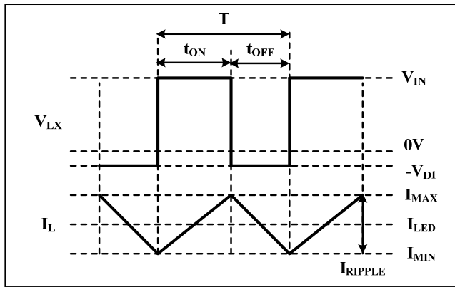
Figure 30 Operating Waveform
