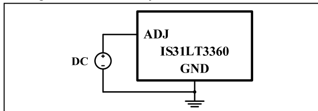
Figure 16 Dimming by External DC Voltage
