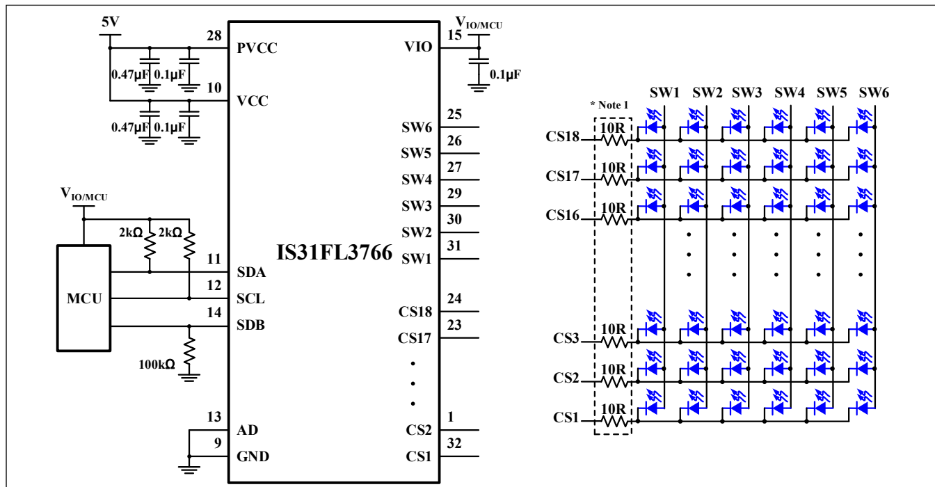
Figure 1 Typical Application Circuit (18x6, LED)
