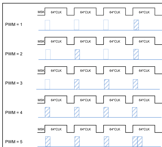
Figure 12 PWMM= “00”, 6+2-bit PWM Mode Enable
