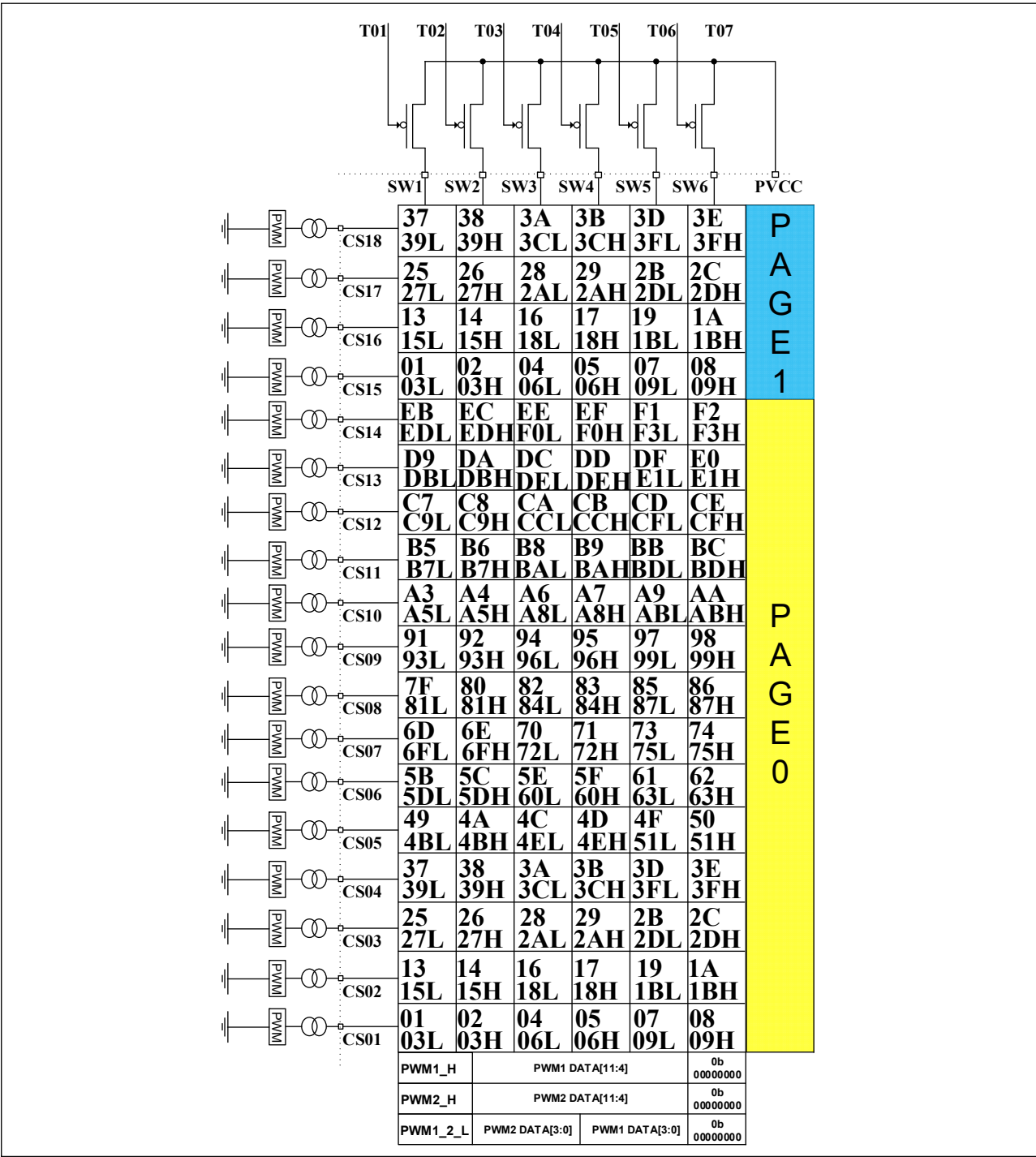
Figure 8 PWM Register
