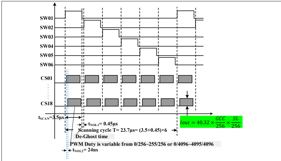
Figure 9 Scanning Timing
