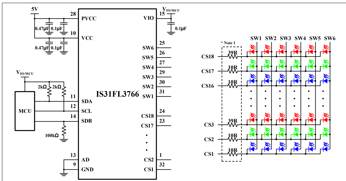
Figure 2 Typical Application Circuit (18x6, RGB)
