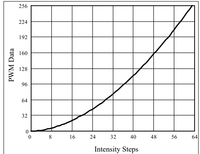
Figure 11 Gamma Correction (64 Steps)
