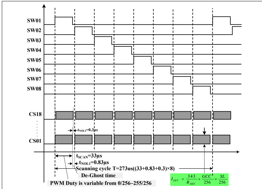
Figure 12 Scanning Timing
