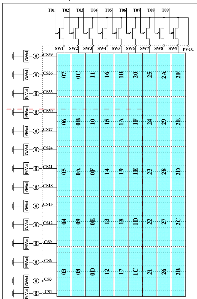
Figure 10 Open/Short Register
