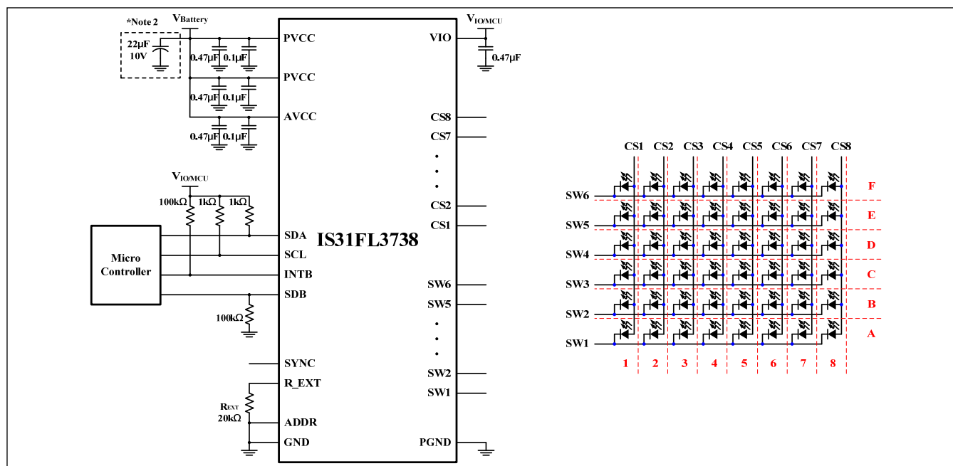
Figure 1 Typical Application Circuit (6×8)
