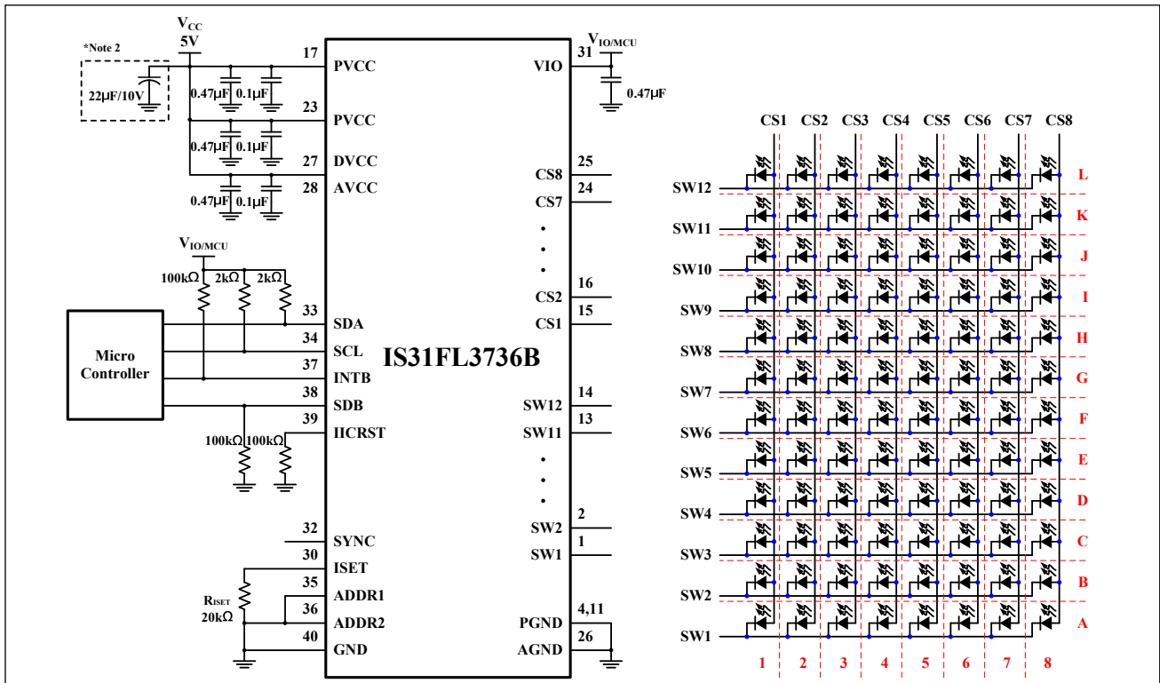
Figure 1 Typical Application Circuit (12x8)
