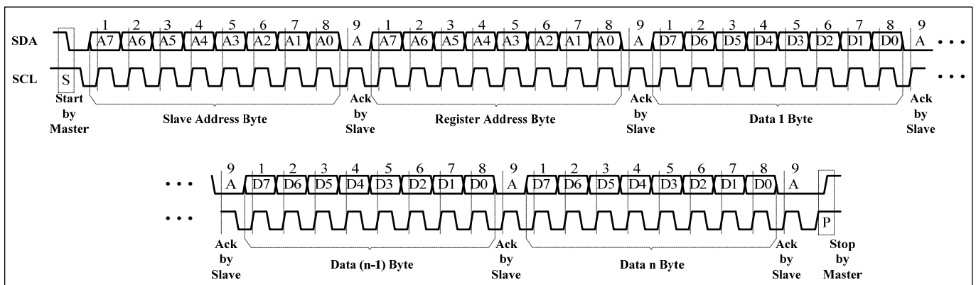
Figure 7 Writing to IS31FL3736B (Automatic address increment)
