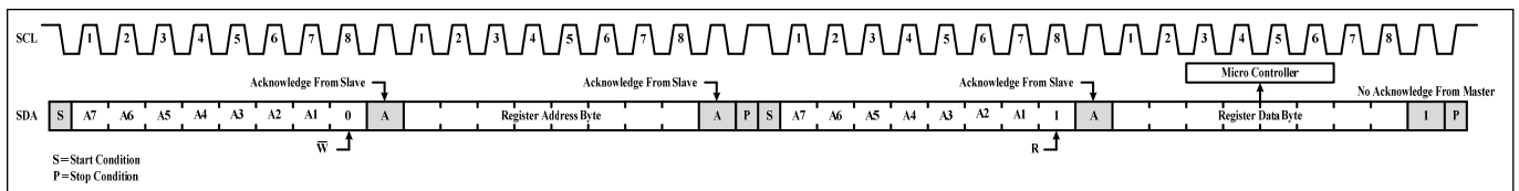
Figure 8 Reading from IS31FL3736B
