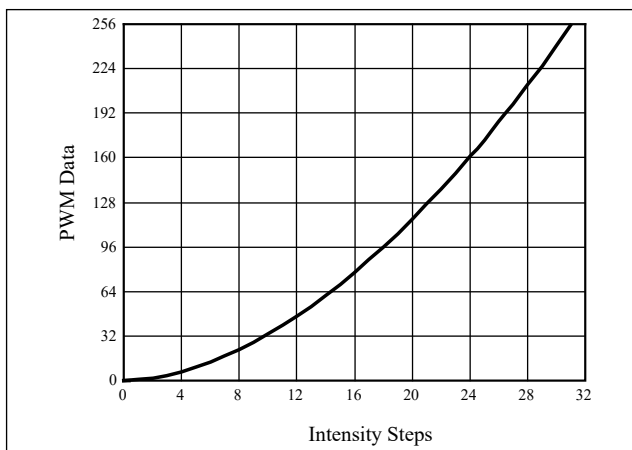
Figure 13 Gamma Correction (32 Steps)
