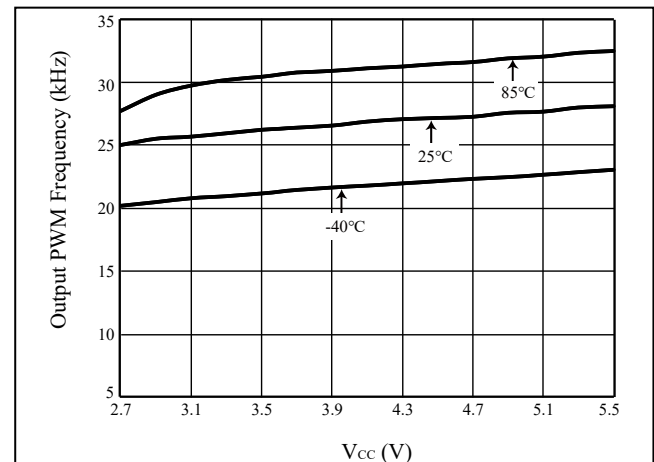
Figure 18 V_{CC} vs. CSx PWM Frequency
