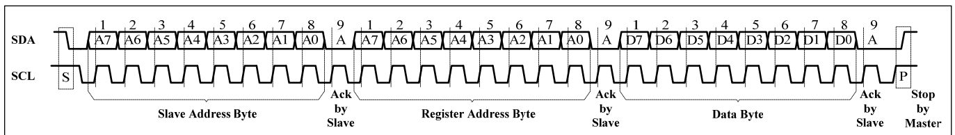
Figure 6 Writing to IS31FL3736B (Typical)
