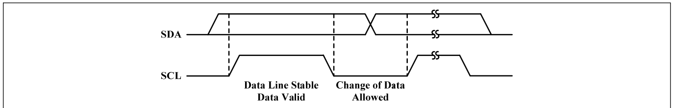
Figure 5 Bit Transfer
