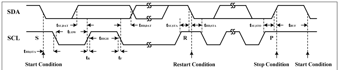
Figure 5 Interface Timing
