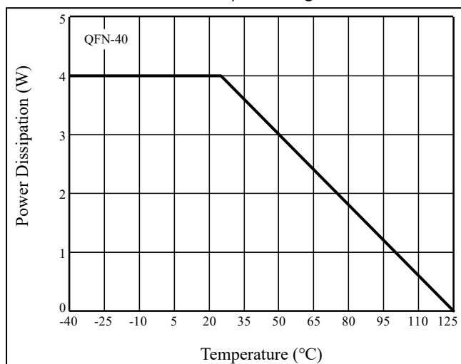
Figure 19 Dissipation Curve
