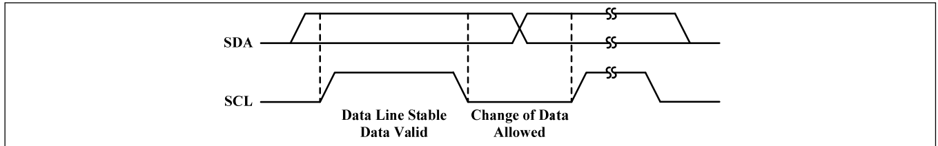
Figure 6 Bit Transfer
