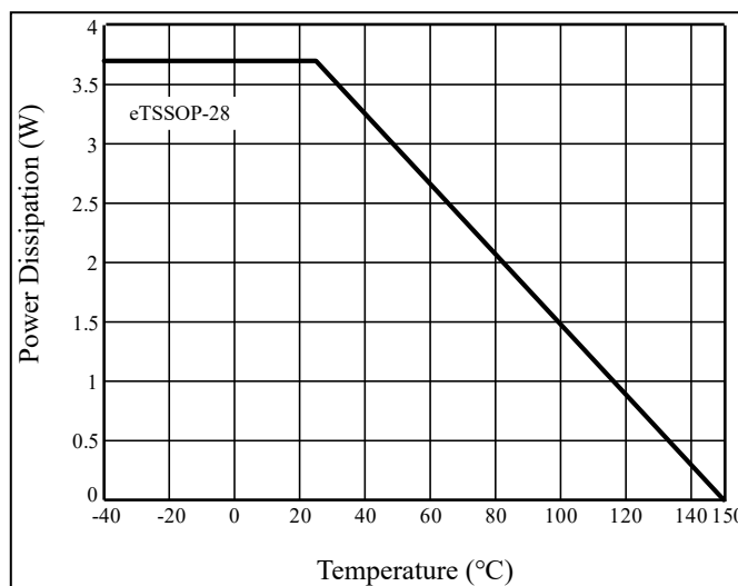
Figure 8 Dissipation Curve
