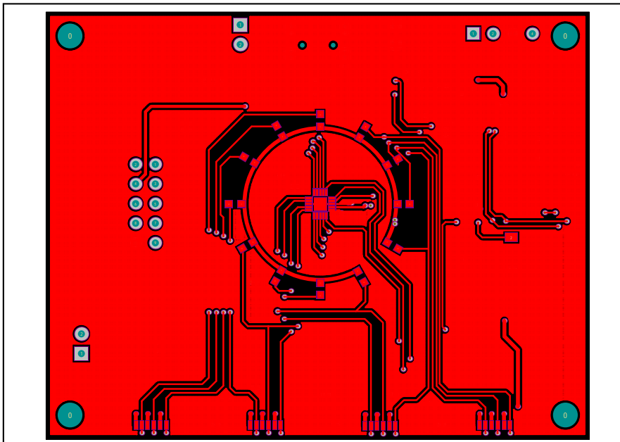
Figure 5: Board PCB Layout - Top Layer
