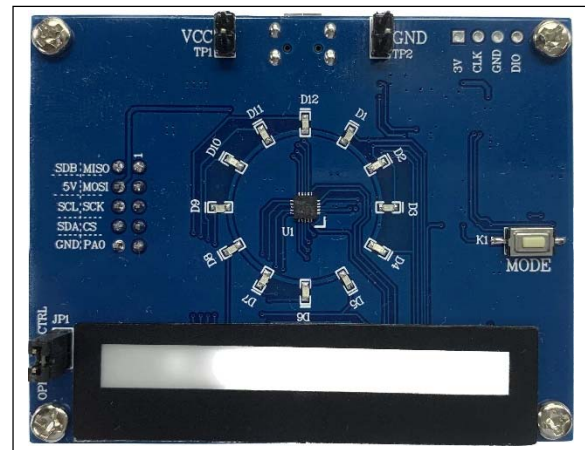
Figure 1: Photo of IS31FL3252 Evaluation Board
