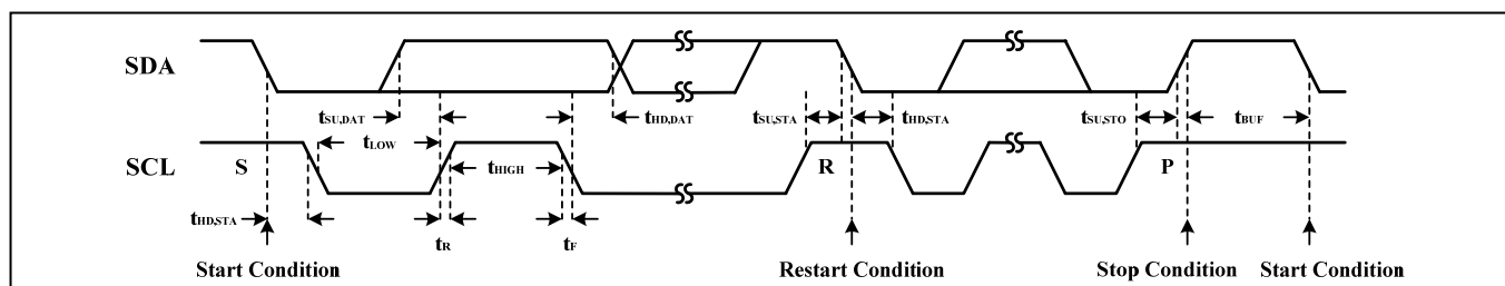
Figure 2 Interface timing
