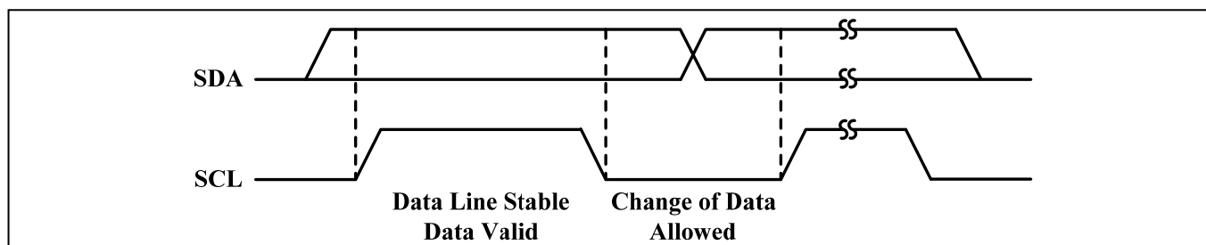
Figure 3 Bit transfer
