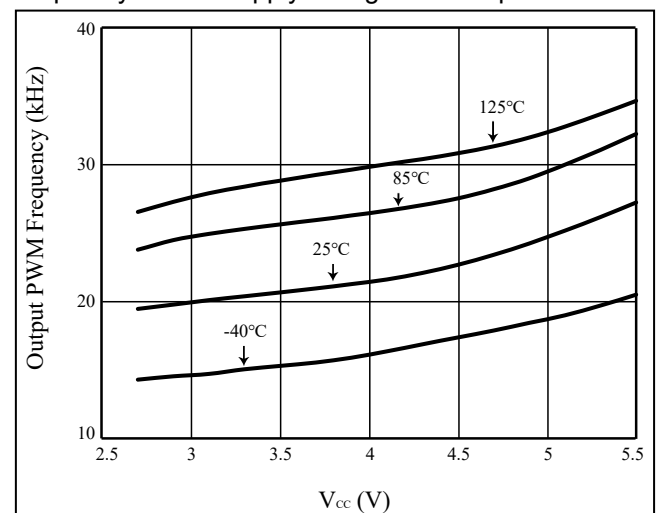
Figure 10 V CC vs. Output PWM Frequency
