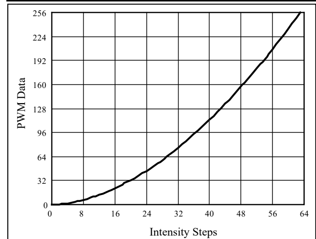
Figure 9 Gamma Correction (64 Steps)
