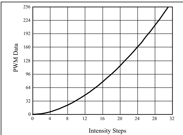
Figure 8 Gamma Correction (32 Steps)
