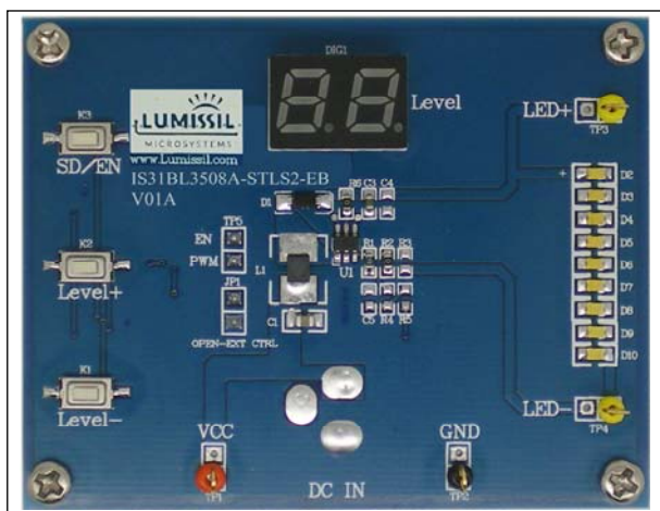
Figure 1: Photo of IS31BL3508A Evaluation Board
