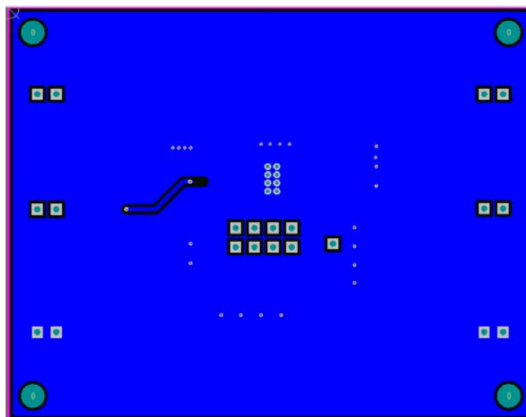
Figure 12 Board PCB Layout - Bottom Layer (SOP-8-EP)
