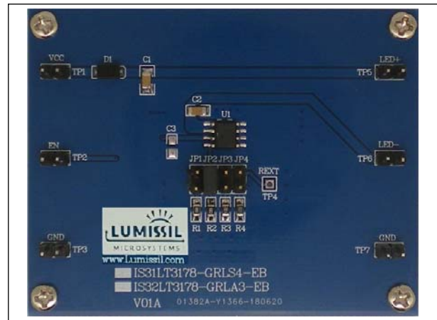
Figure 2 Photo of IS31LT3178-GRSL4/IS32LT3178-GRLA3 Evaluation Board
