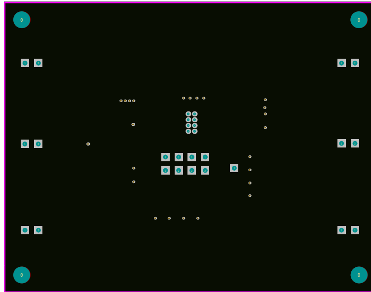
Figure 11 Board Component Placement Guide - Bottom Layer (SOP-8-EP)
